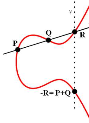
Figure 2.1: Addition of points on an elliptic curve
