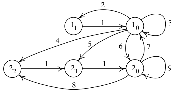
FIGURE 1. The graph \Gamma_{P(t)} for Example 3.1
